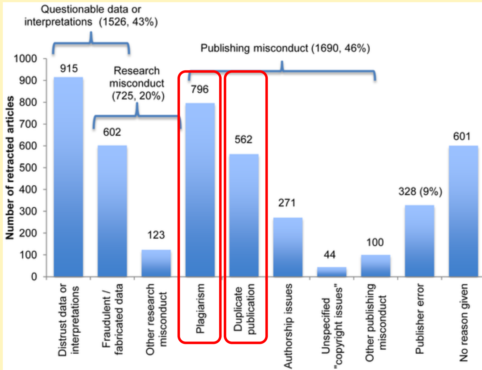
Figure 3. Justifications for retraction stated in the notices consulted, which accounted for 4,232 retracted articles.
