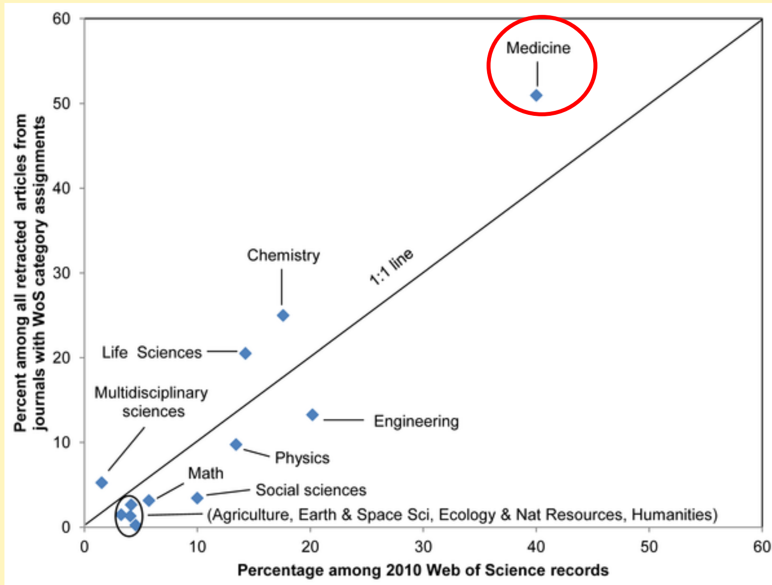
Figure 2. Percentage of retractions vs. percentage of 2010 Web of Science records among 12 broad scholarly fields.
